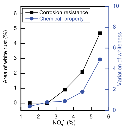
Fig. 2 Corrosion resistance and chemical property according to the concentration of \text{NO}_3^- .
