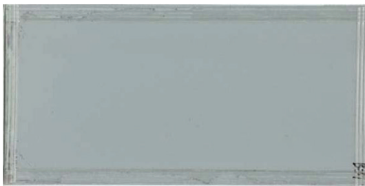
Photo 2 Surface appearance of antibacterial antifinger-resin coated steel sheet after SST 96 hours.
